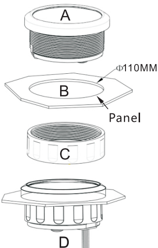
Picture B: Before installation, firstly, to open a hole \Phi 110\text{mm} (4-3/8") of the panel, make sure there is a space with(55mm backyard of panel) as well.
